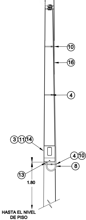
VISTA FRONTAL
